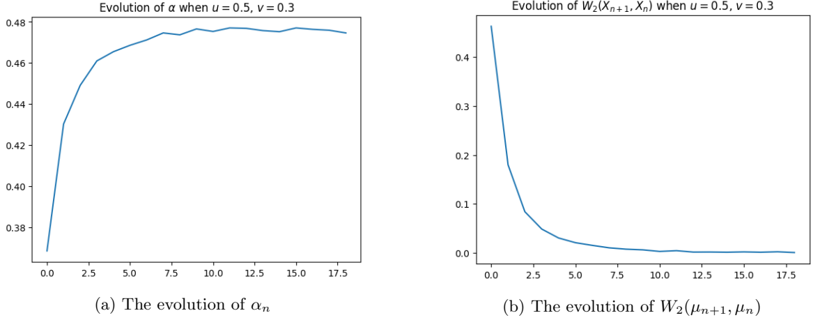
Figure 4.4: Results of the mean-preserving recurrence (4.21) with u = 0.5 and v = 0.3
