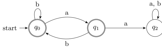
Figure 2.1: DFA recognizing strings over \{a, b\} that do not contain aa .
