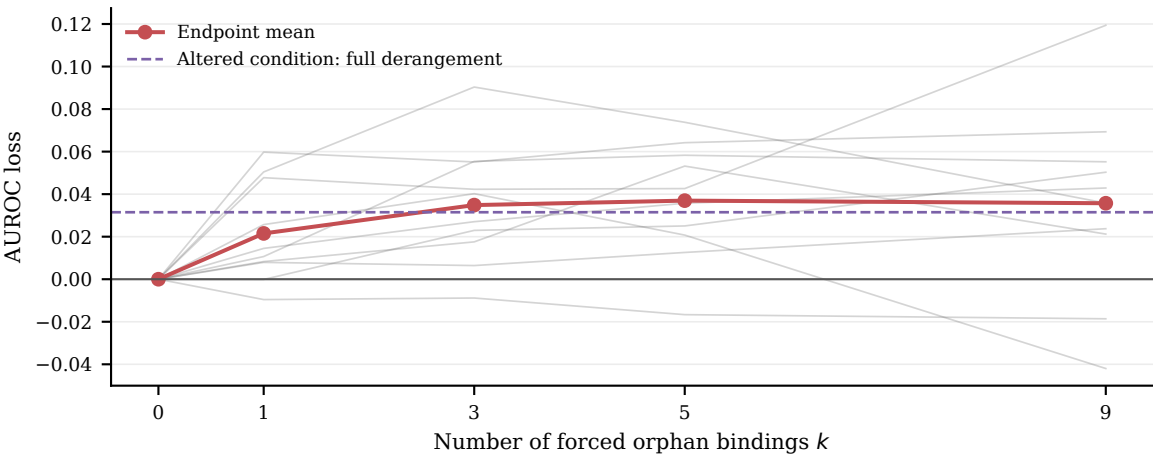
Performance loss from forced plausible-neighbour bindings
