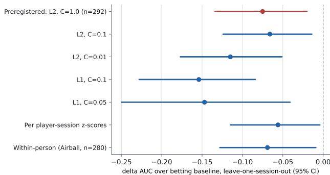
Fig. 3. No analysis choice rescues the features (round 1: pooled LOSO over the four round 1 sessions). All arms are \Delta AUC over the betting baseline for is_weak with hand-grouped bootstrap 95% CIs.
