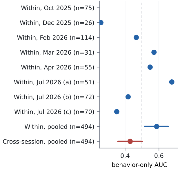
Fig. 5. Session locality, resolved on eight sessions (round 2). Within-session grouped cross-validation finds real but heterogeneous behavioral signal (pooled CI excludes chance); the same features transfer at or below chance across sessions.
