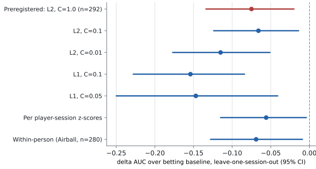
Fig. 2. No analysis choice rescues the features. All arms are \Delta AUC over the betting baseline for is_weak , pooled LOSO, hand-grouped bootstrap 95% CIs.
