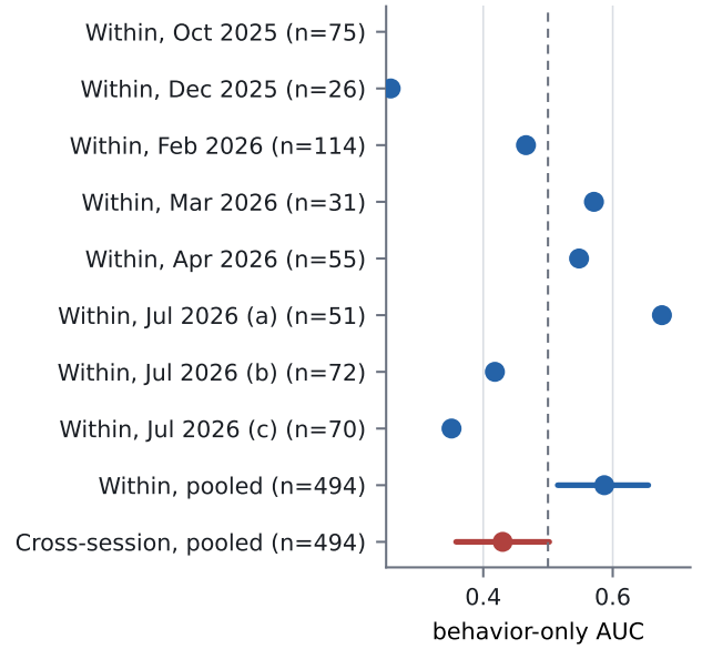
Fig. 4. Session locality, resolved on eight sessions (round 2). Within-session grouped cross-validation finds real but heterogeneous behavioral signal (pooled CI excludes chance); the same features transfer at or below chance across sessions.
