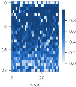
MeshXL on meshes mean 0.660
