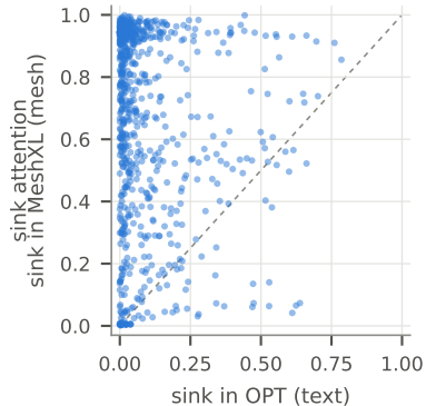
same head, both models \rho = -0.146
