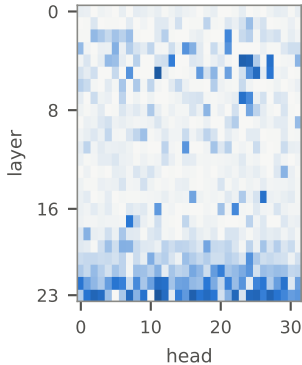
OPT-1.3b on text mean 0.094
