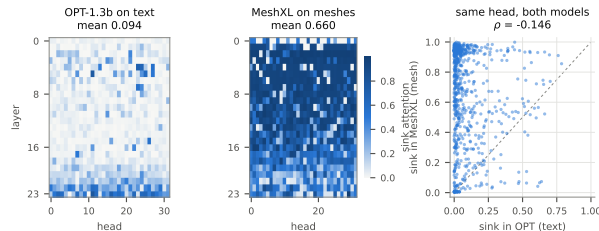
Figure 5: Same transformer body, unrelated sink structure. MeshXL inherits OPT-1.3b’s weights and reinitializes only the embeddings, yet 72% of its heads sink above 0.5 against 4% of OPT’s, and the per-head maps do not correspond.
