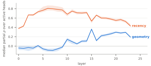
Figure 2: Recency dominates at every depth. Geometry is absent or slightly negative through layer 9 and emerges only in the second half of the network, which inverts the usual reading of layer-wise geometric specialization. Bands are bootstrap 95% intervals over chairs.
