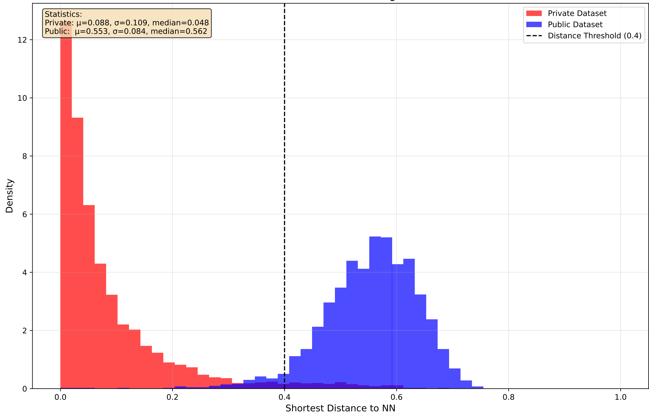
Distribution of Shortest Distances During KNN-LM Generation
