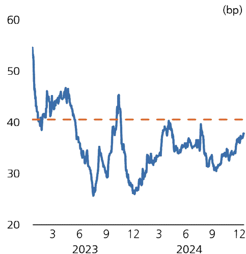
CDS프리미엄
