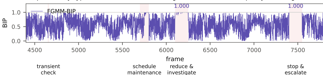
(c) probability-type index: saturated on both ghosts — a BIP-driven policy cannot grade them
