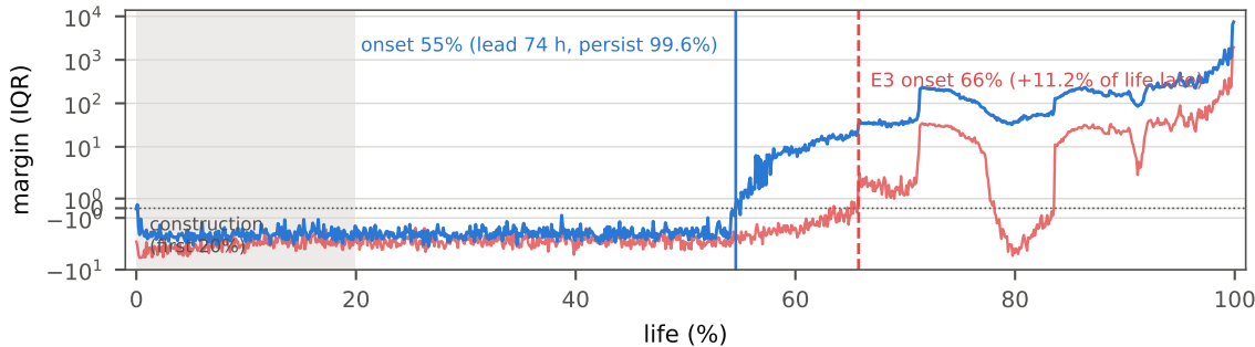
IMS test 2 — bearing 1 (outer race)
