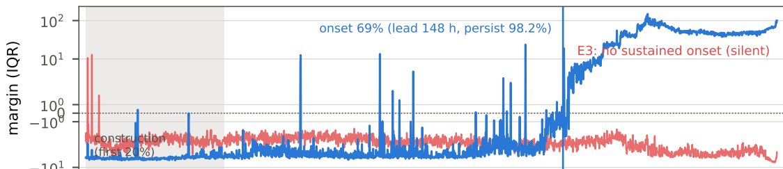
IMS test 2 — bearing 1 (outer race)
