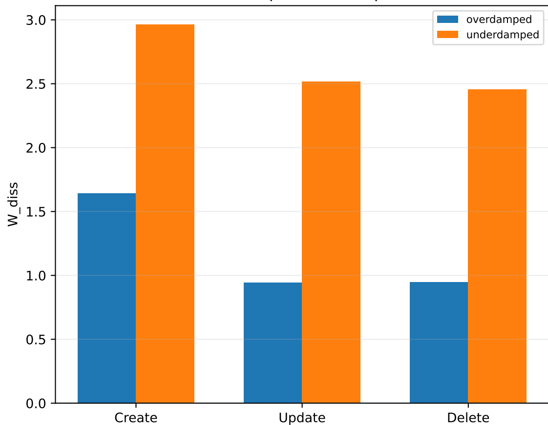
Protocol-dependent dissipation
