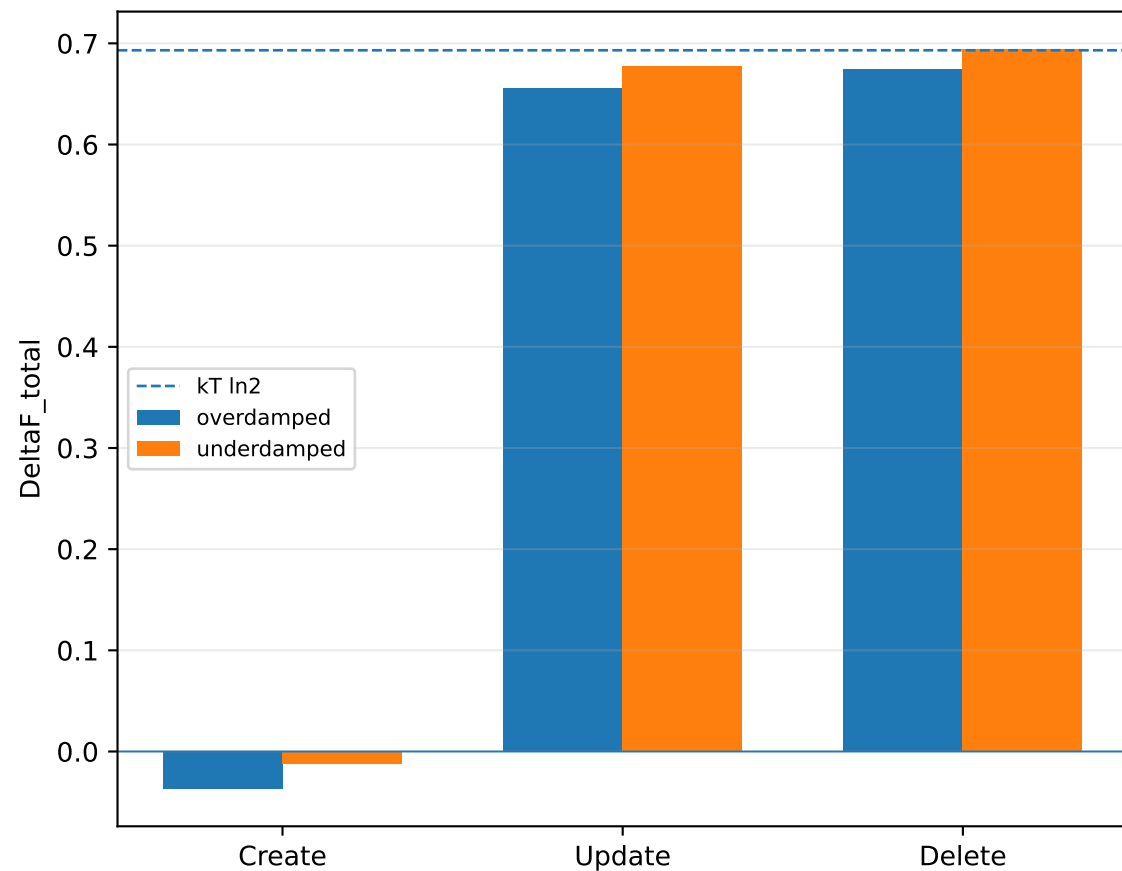
State-function classification
