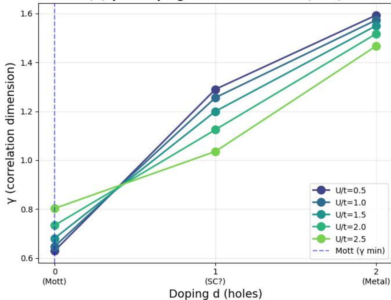
(a) \gamma vs Doping: Minimum at Mott ( d=0 )
