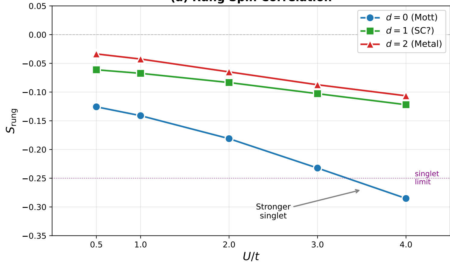
(a) Rung Spin Correlation
