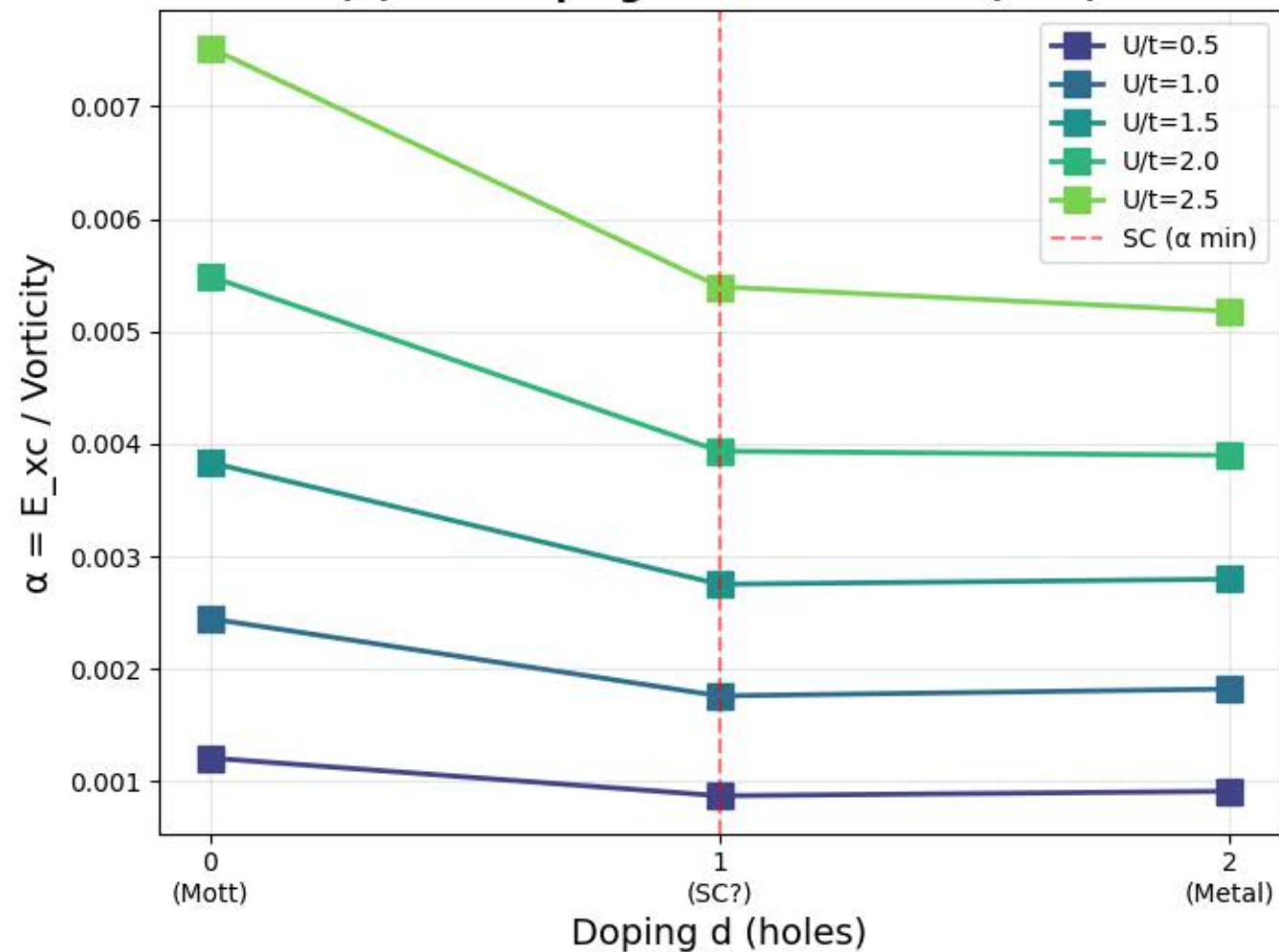
(a) \alpha vs Doping: Minimum at SC ( d=1 )
