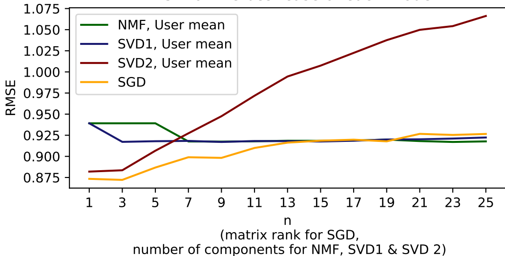
RMSE for the best case of each model
