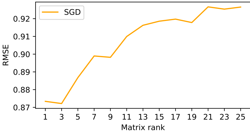
RMSE for SGD model
