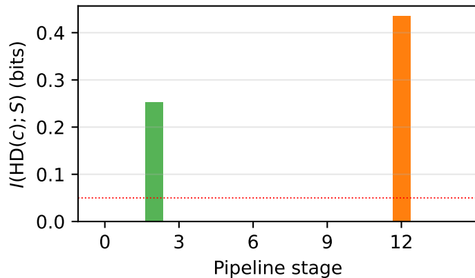
MI on power trace ( d = 2 )
