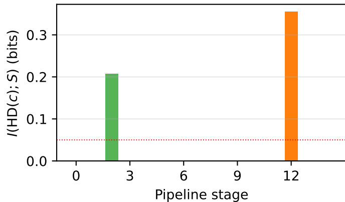
MI on power trace ( d = 1 )
