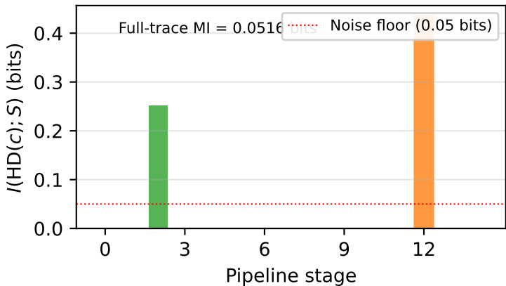
Per-stage MI on power trace ( d = 2 )
