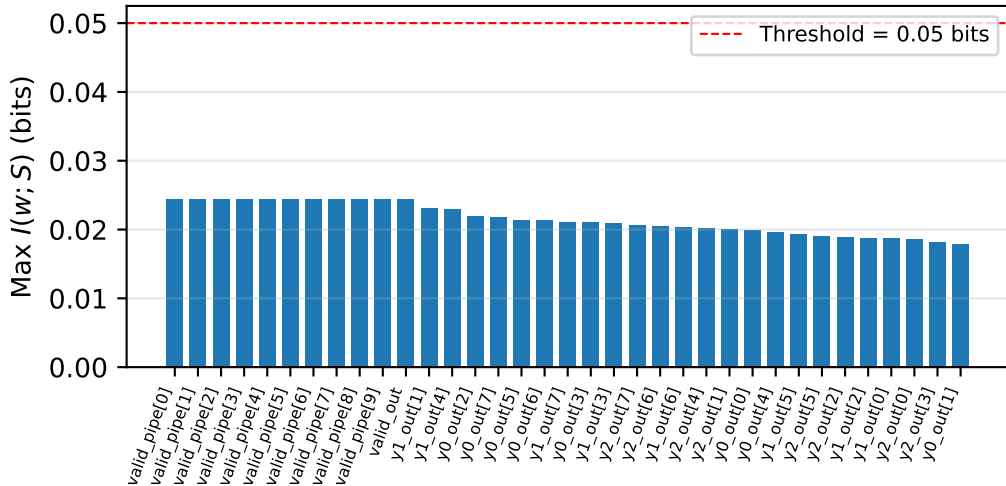
Per-wire mutual information ( d = 2 )
