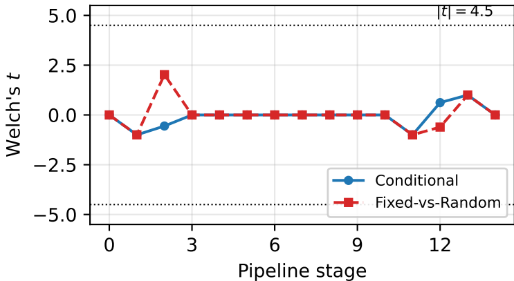
TVLA per-stage t -statistic ( d = 1 )
