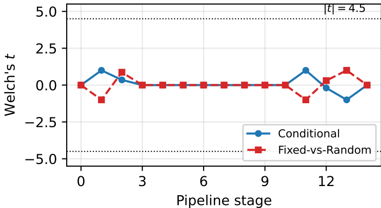
TVLA per-stage t -statistic ( d = 2 )
