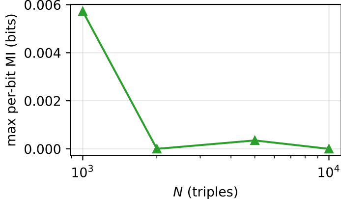
MI per-bit at output cycle (order 2)
