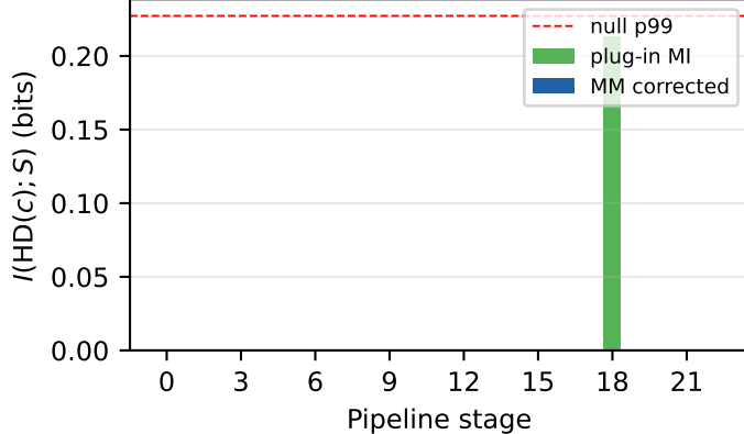
MI on power trace ( d = 1 ), corrected HD
