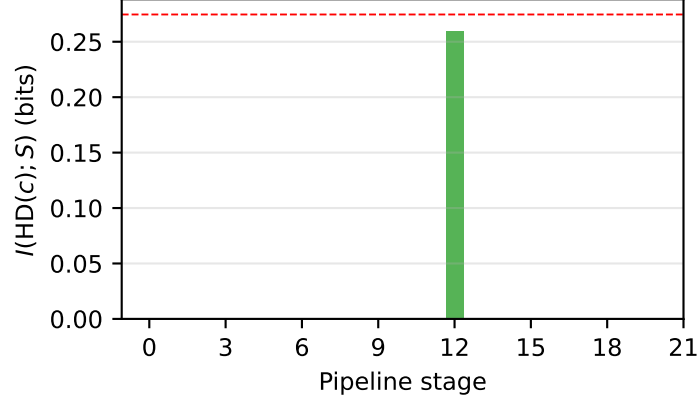
MI on power trace ( d = 2 ), corrected HD
