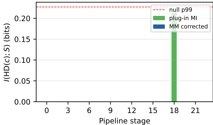
MI on power trace ( d = 1 ), 23-stage window
