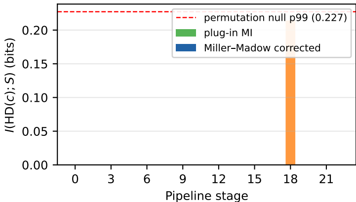
Per-stage MI on power trace ( d = 1 ), corrected HD
