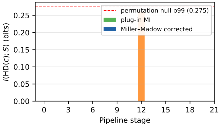
Per-stage MI on power trace ( d = 2 ), corrected HD
