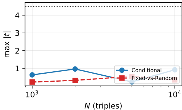
(c) TVLA max |t| ( d = 1 )
