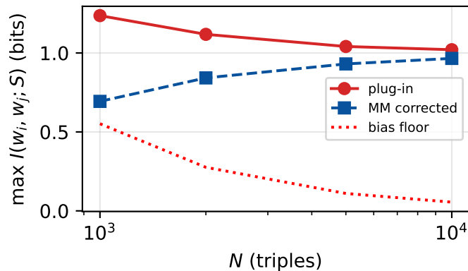
(b) 2-wire joint MI ( d = 1 )
