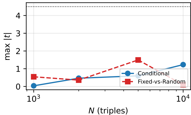
(c) TVLA max |t| ( d = 2 )
