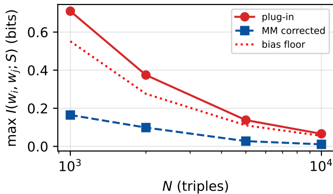
(b) 2-wire joint MI ( d = 2 )
