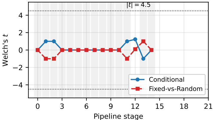
TVLA per-stage t -statistic ( d = 2 ), corrected HD
