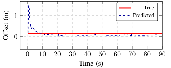
Fig. 5. Predicted payload offset over-time on X-axis at 2 nd episode
