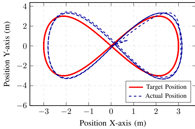
Fig. 7. Target position and actual position at 2 th episode
