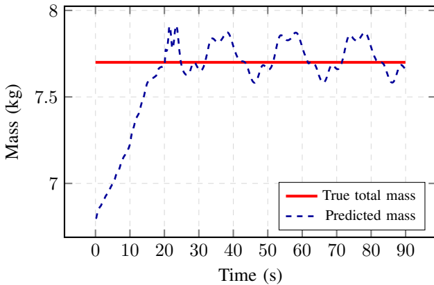
Fig. 2. Mass prediction over-time at 2 st episode
