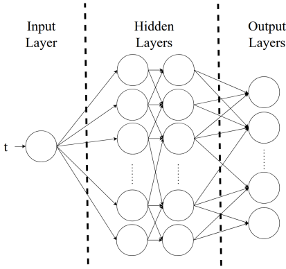
Fig. 1. The proposed PINN architecture based on a fully connected ANN. The input layer accepts continuous time t , which is propagated through two hidden layers comprising 64 neurons each. The output layer yields the 12-dimensional kinematic state vector of the composite body defined in Eq. (16). A hyperbolic tangent ( \tanh ) activation function is employed across all hidden layers.
