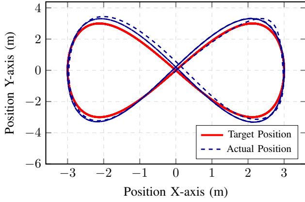
Fig. 2. The body is able to follow the desired trajectory without crashing at 1 st episode
