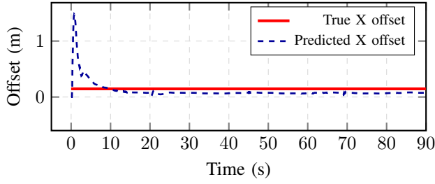
Fig. 6. Predicted payload offset over time along the X-axis during the 2 nd episode. The network's ability to rapidly converge upon the true offset during the initial takeoff transient demonstrates converging parameter estimation without the requirement for persistent excitation.
