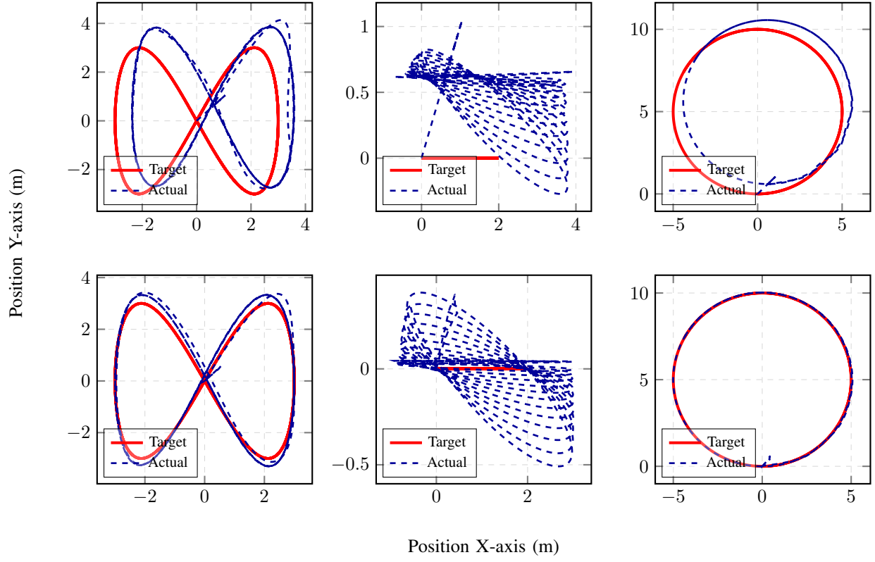
Fig. 1. Trajectory tracking performance in the X-Y plane for each trajectory divided by columns in order Figure-8, lawn mower, and circular path. The top row illustrates the network performance with 0 weight of physics loss, while the bottom row demonstrates the improved trajectory using the proposed method.
