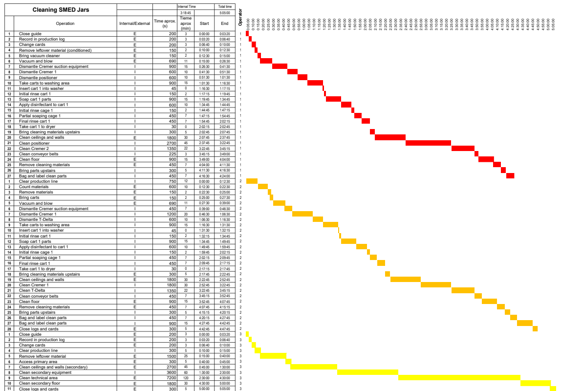
Figure 4: Gantt Diagram of Cleaning Procedure
