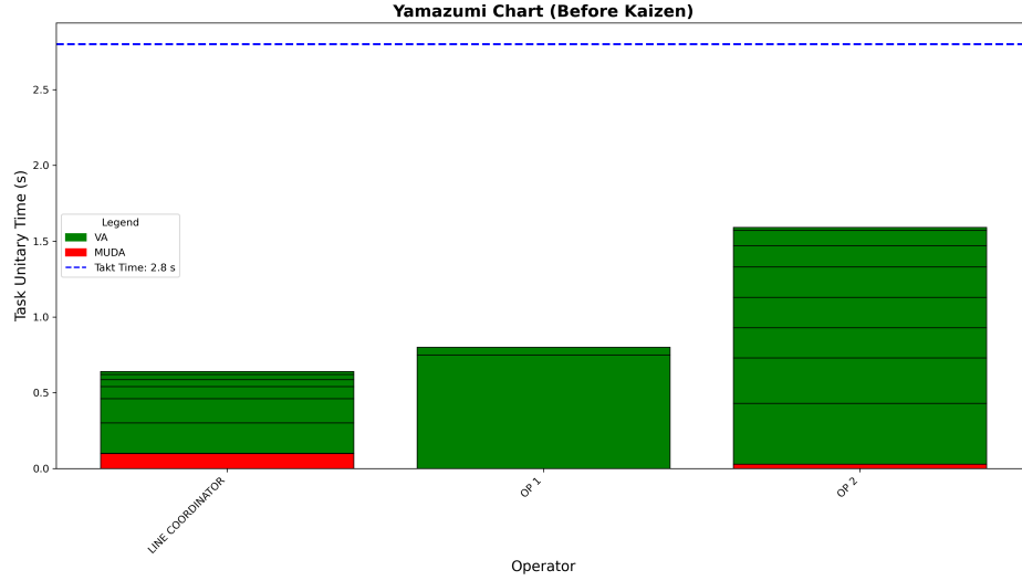
Figure 20: Yamazumi Chart Showing Task distribution before improvement.
