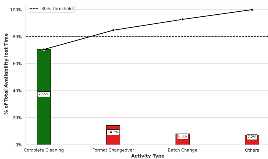
Figure 11: Pareto Chart of Main Losses on Availability. In Green Above 80% of cumulated time, in Red the rest 20% of time
