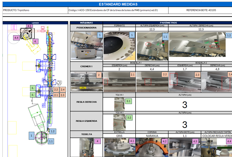
Figure 14: OPL showing measures and placement for machine parts after cleaning.
