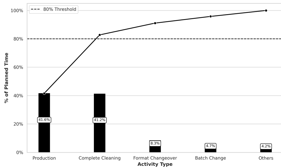
Figure 10: Pareto Chart of Planned Time dedication by Activity
