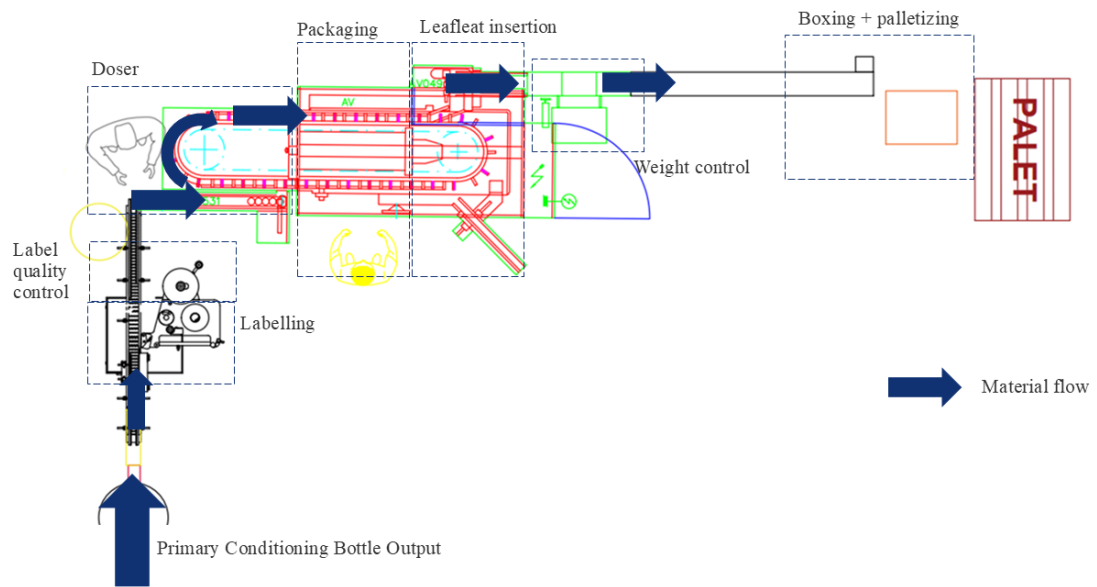
Figure 18: Detailed layout and material flow in the Liquids Line.
