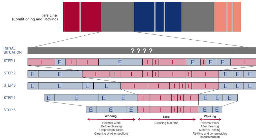
Figure 12: Detailed application overview of the SMED Methodology applied to the pilot line.
