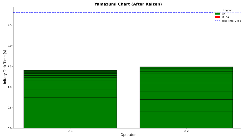
Figure 22: Yamazumi Chart Showing Task distribution with 2 operators.
