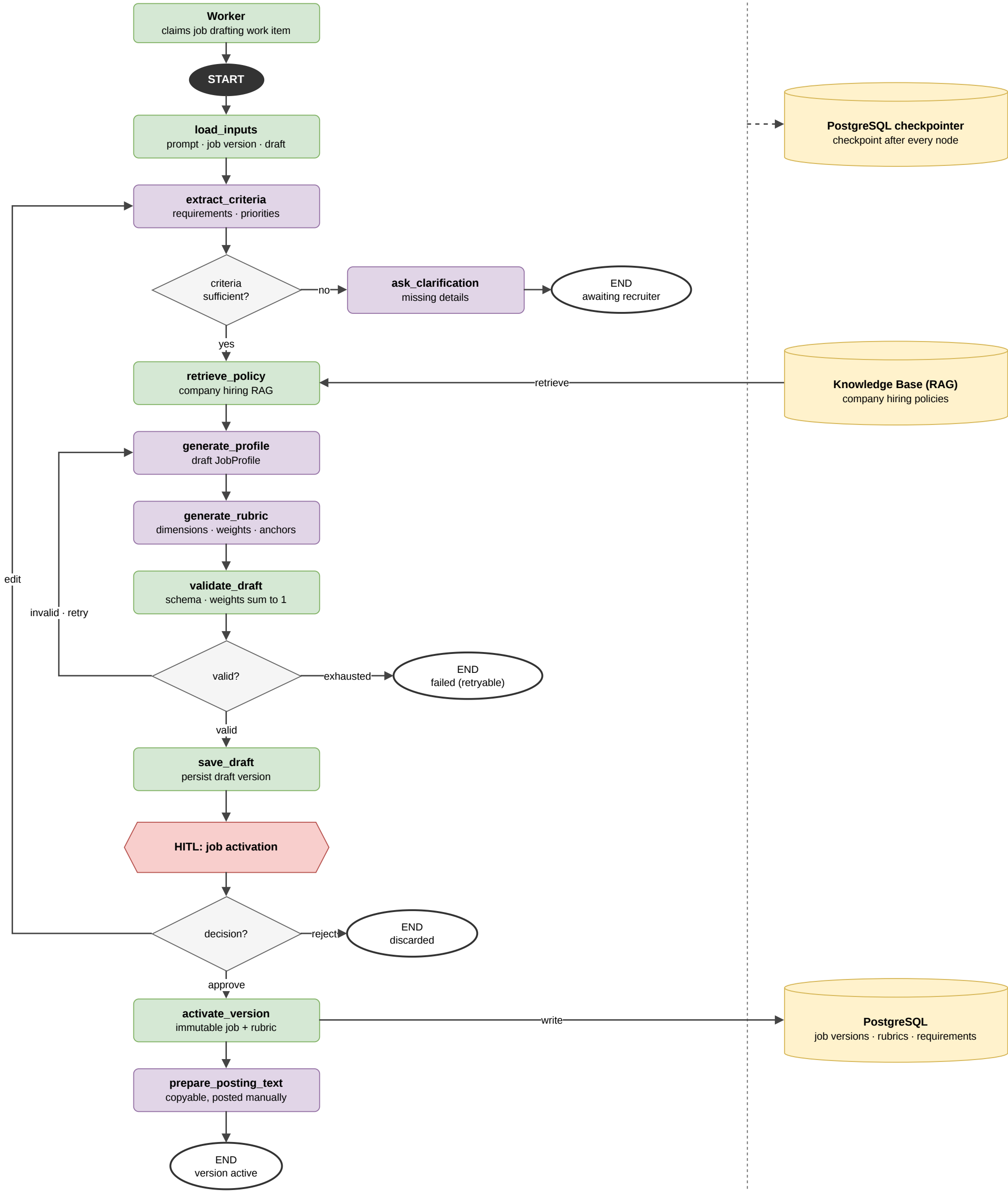
LangGraph run — job intelligence graph
