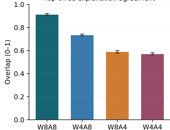
Top-three explanation agreement
