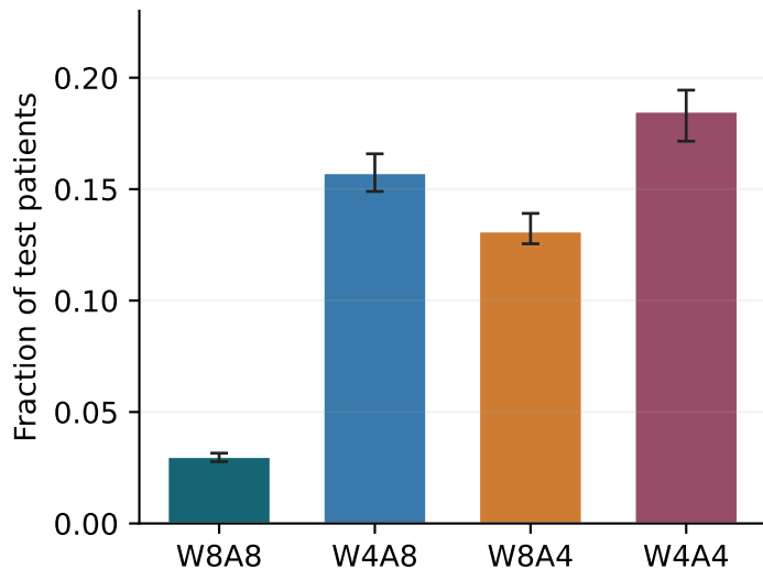
Decisions crossing FP32 threshold
