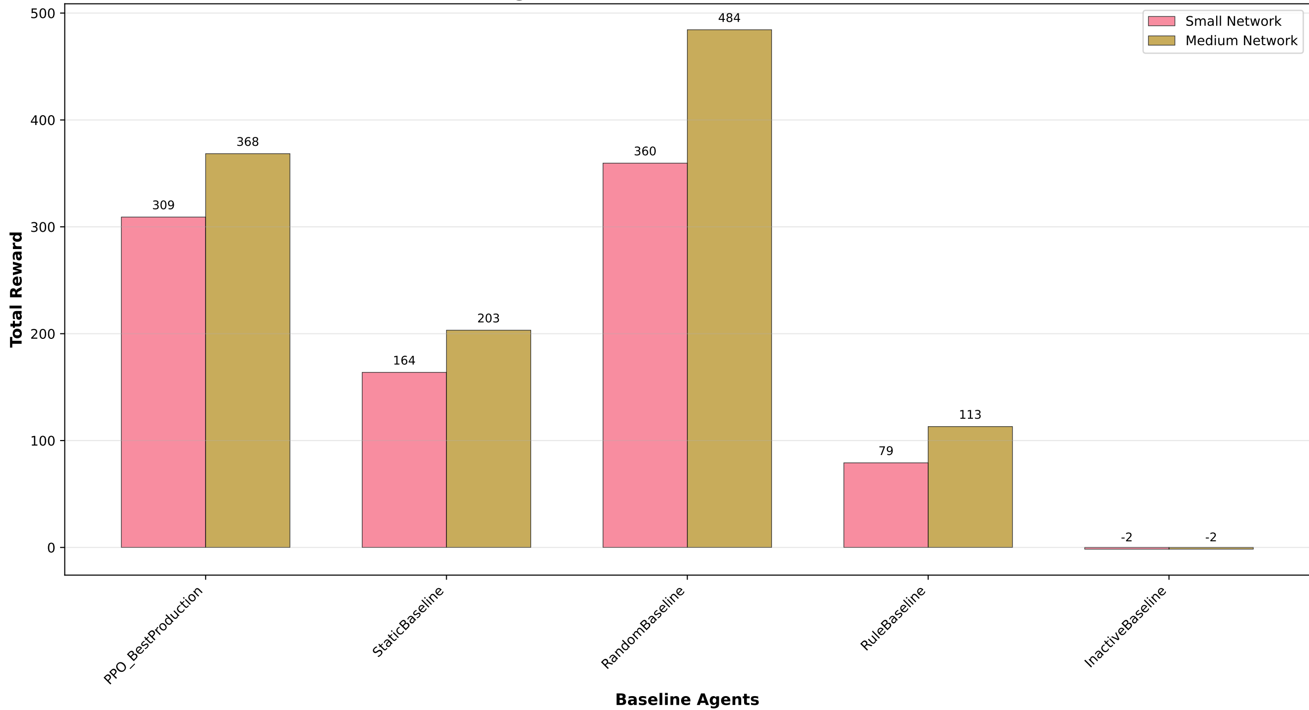
Baseline Agent Performance Across Environments
