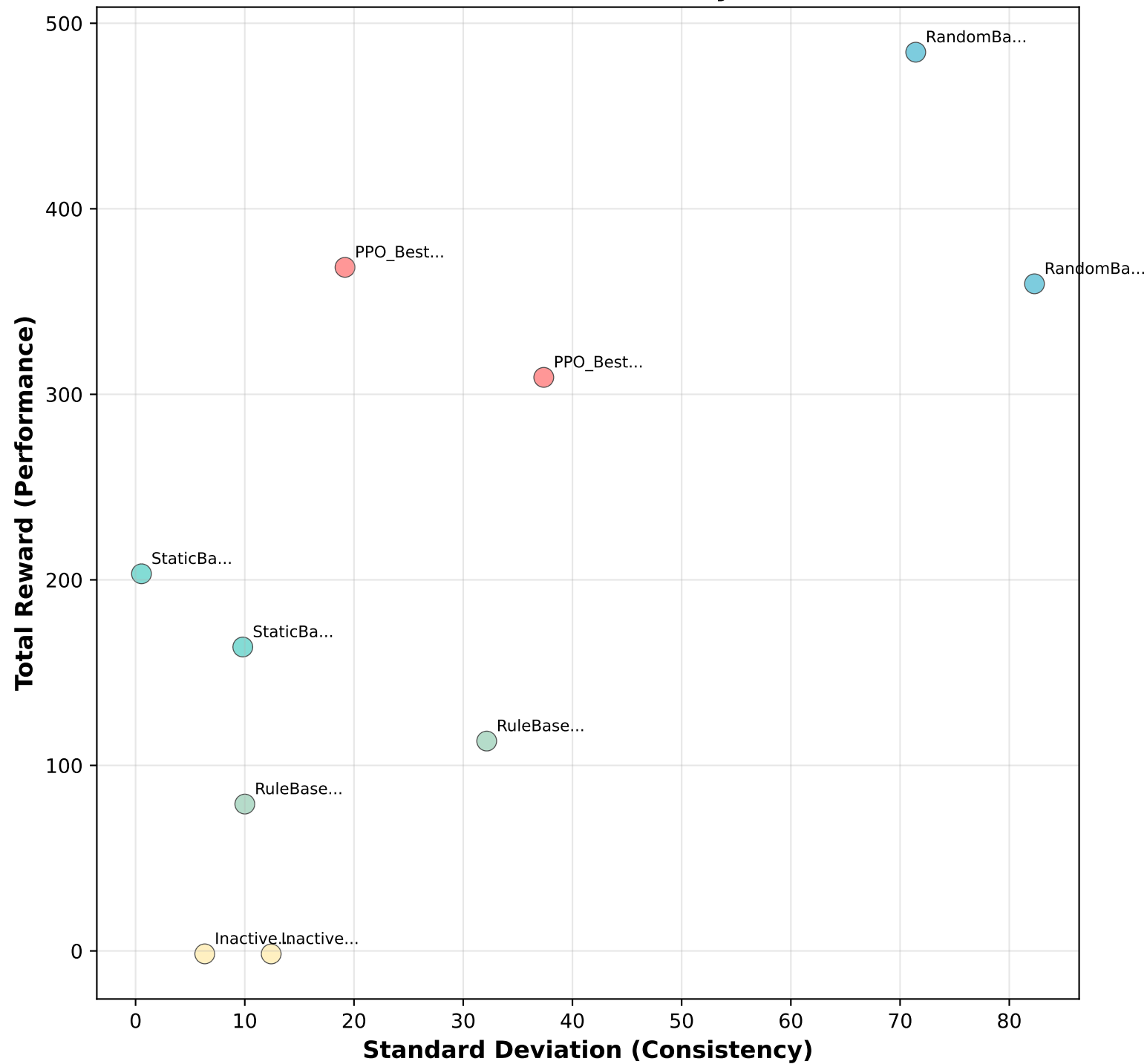
Performance vs Consistency Trade-off
