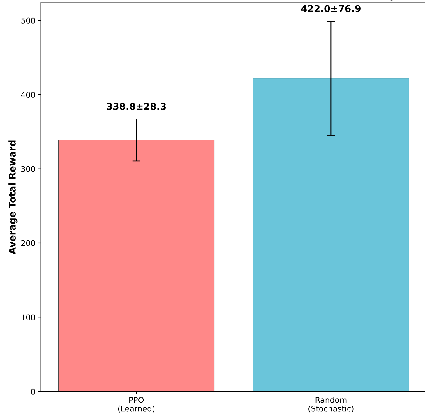
PPO vs RandomBaseline: Performance & Consistency
