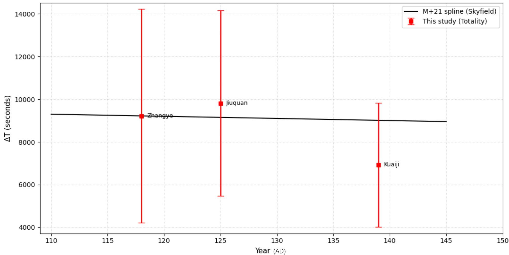
\Delta T Constraints from Historic Total Solar Eclipses
