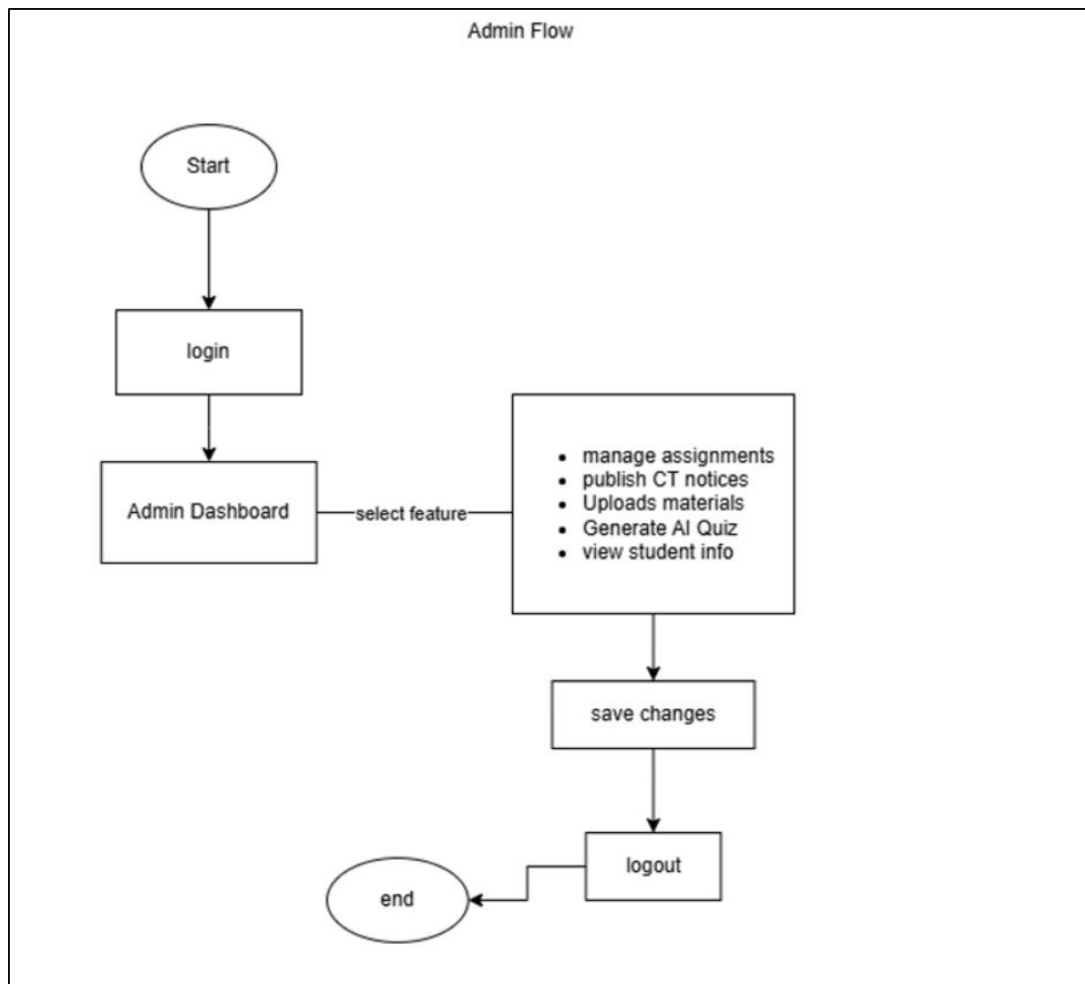
Fig-3: Admin flow design
