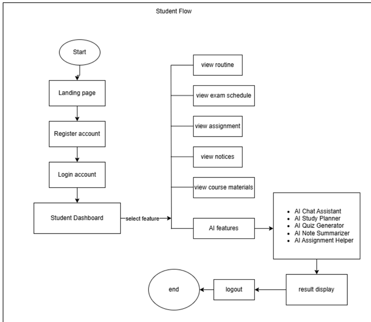
Fig-1: Student flow design
