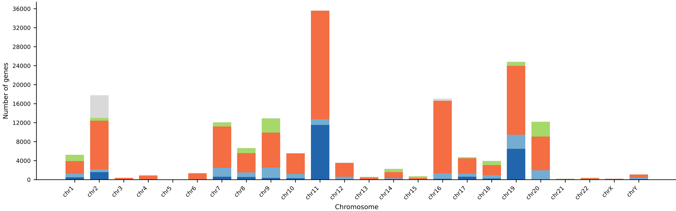
Gene biotypes in centromeric regions — by chromosome
