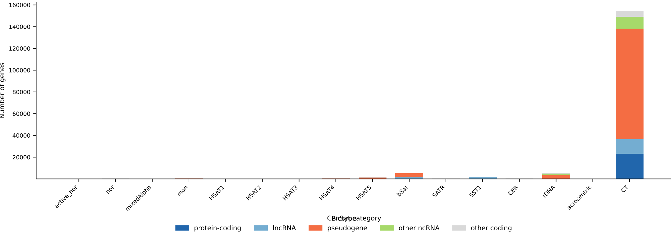
Gene biotypes in centromeric regions — by satellite class
