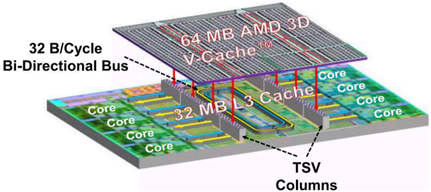
Fig. 6: AMD's implementation of vertical cache [11].
