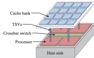
Fig. 5: A depiction of how cache is layered using TSVs [10].
