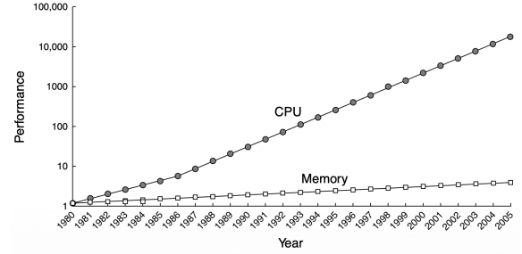
Fig. 4: The speedup of CPU processors compared to main memory [7].
