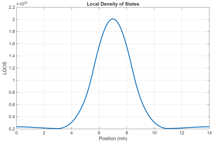
Figure: Local density of states along the growth direction of a double-barrier resonant structure at an energy lying inside the well, evidencing the standing-wave pattern of the quasi-bound state. ( U_{barr} = 0.25 eV, t_{barr} = 2.5 nm)
