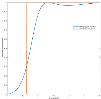
Figure: Transmission coefficient of a thick barrier. ( t_{barr} = 4.5 nm)
