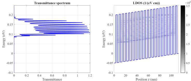
Figure: Same lattice ( t_{\text{barr}} = 2.5 nm) under an applied bias of V = 0.05 V. ( U_{\text{barr}} = 0.25 eV, t_{\text{barr}} = 2.5 nm, t_{\text{well}} = 3 nm)
