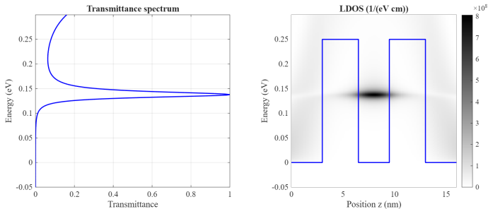
Figure: Double barrier with increased barrier thickness. ( U_{barr} = 0.25 eV, t_{barr} = 3.5 nm, t_{well} = 3 nm)
