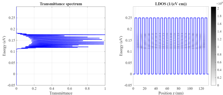
Figure: Transmittance spectrum (left) and LDOS map (right) for an unbiased 20-period superlattice ( t_{\text{barr}} = 3.5 nm), showing flat minibands extending uniformly across the device. ( U_{\text{barr}} = 0.25 eV, t_{\text{barr}} = 3.5 nm, t_{\text{well}} = 3 nm)
