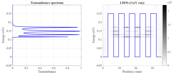
Figure: Same conditions, 5 barriers: the single resonance splits into a miniband of 5 closely spaced resonances. ( U_{barr} = 0.25 eV, t_{barr} = 3.5 nm, t_{well} = 3 nm)
