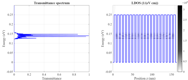
Figure: Same conditions, but with wider barriers ( U_{barr} = 0.25 eV, t_{barr} = 5 nm, t_{well} = 3 nm)
