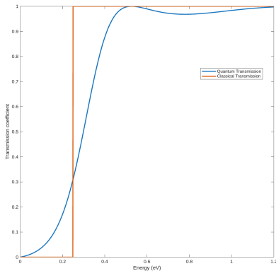
Figure: Transmission coefficient of a thick barrier
