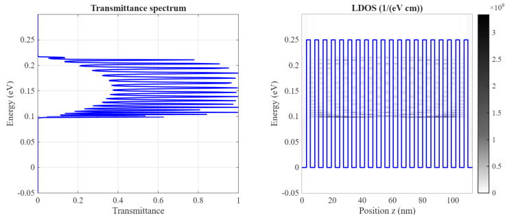
Figure: Same conditions, but with wider barriers ( t_{\text{barr}} = 5 nm)
