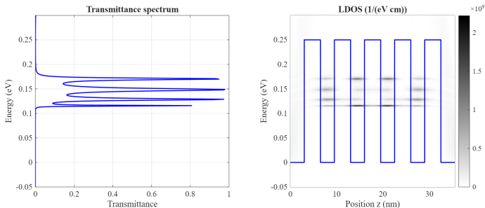
Figure: Same conditions, 5 barriers: the single resonance splits into a miniband of 5 closely spaced resonances.
