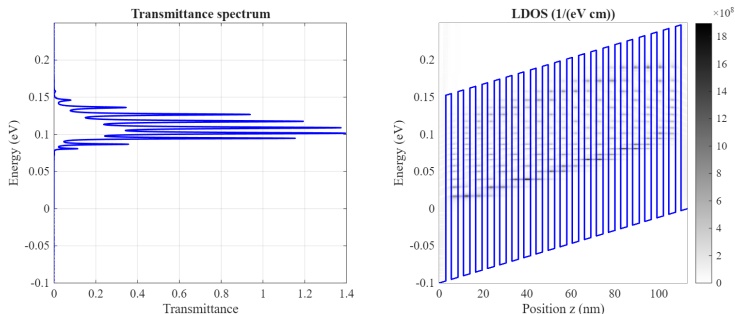
Figure: Same quantities for a 20-period superlattice ( t_{\text{barr}} = 2.5 nm) under an applied bias of V = 0.1 V: the linear potential drop tilts the minibands and breaks the resonant alignment between adjacent wells (note that t_{\text{barr}} differs from the unbiased case in the previous slide, so the comparison is qualitative).
