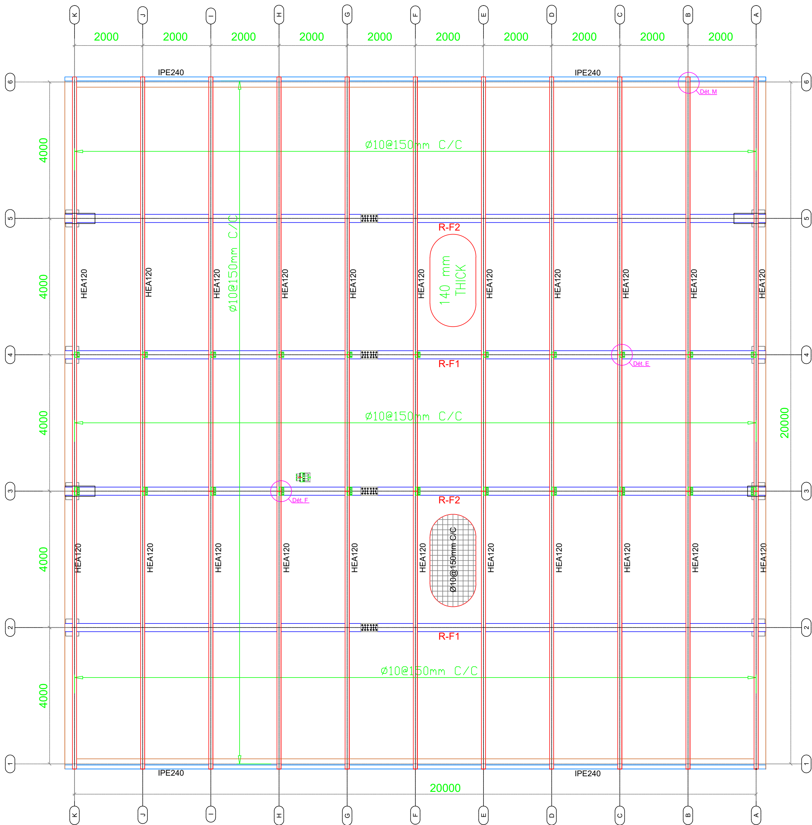
UPPER ROOF AUDITORIUM FRAMING
