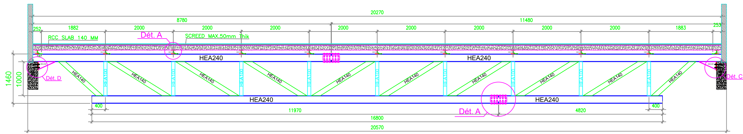
ELEVATION-STEEL TRUSS R-F1
