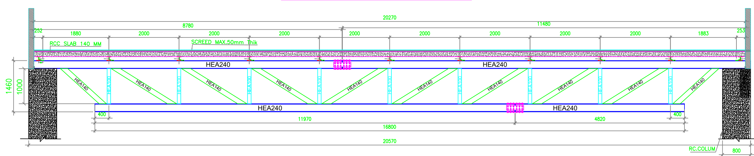
ELEVATION-STEEL TRUSS R-F2
