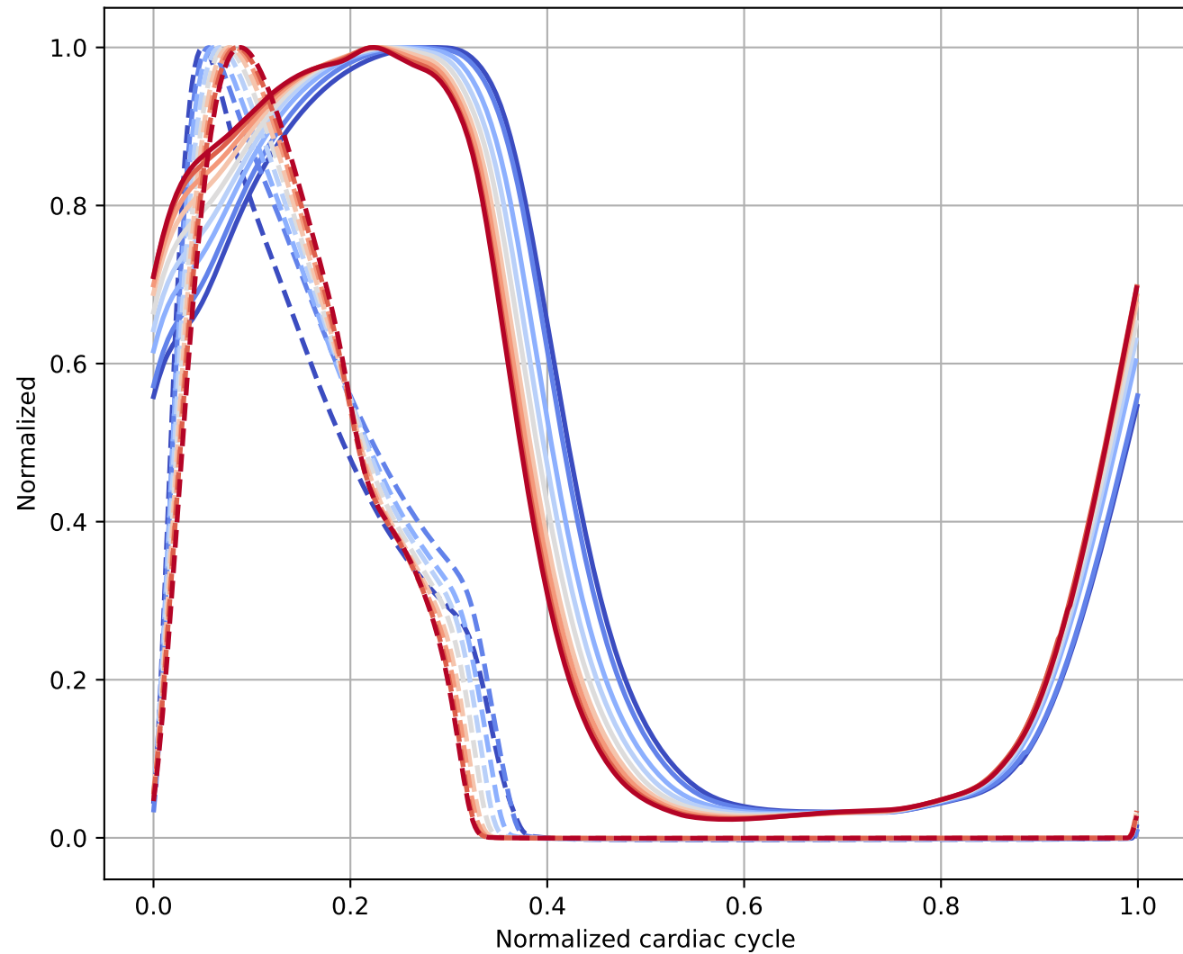
RV pressure + flow
