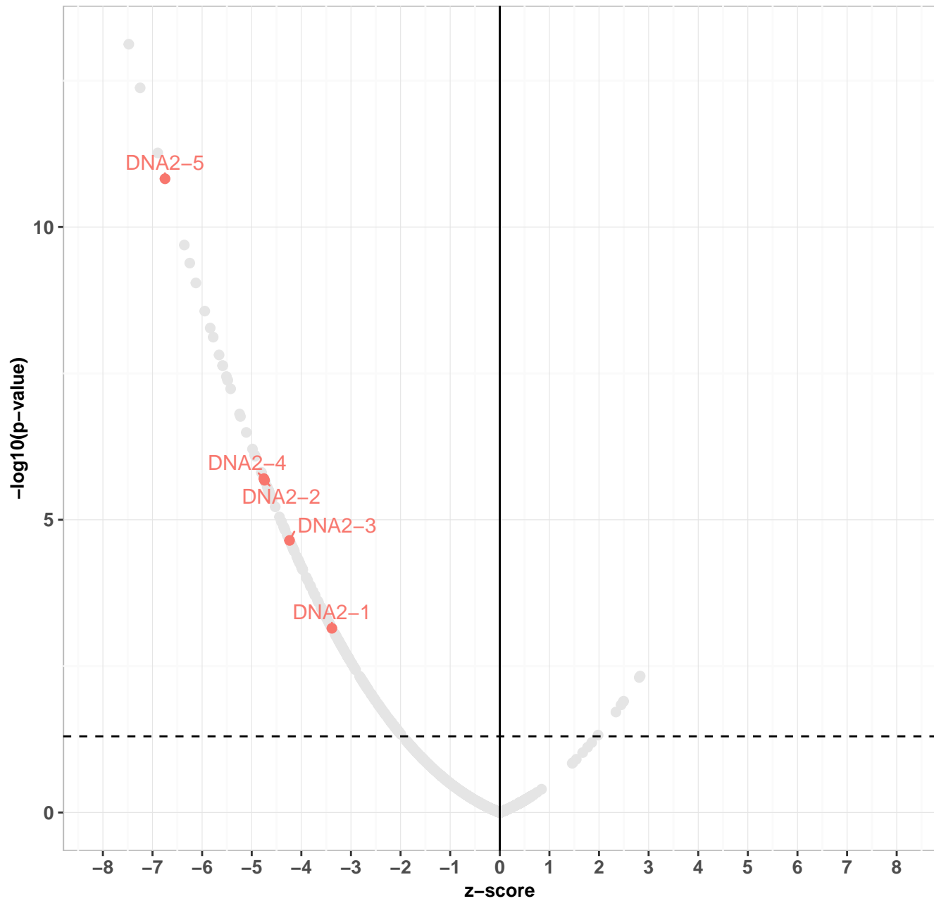
t7 vs t0, neg. sel. Top 15: drugZ results
