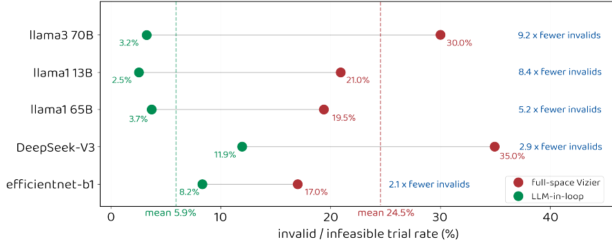
Figure 8: Invalid/infeasible trial rate (%) for full-space Vizier vs. LLM-in-loop across five workloads. The LLM Architect reduces the mean invalid rate from 24.5% to 5.9% ( 4.1\times reduction), with the largest gains on LLM workloads where the hardware search space is most prone to infeasible configurations.
