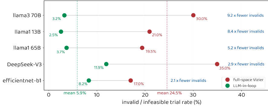
Figure 8: Invalid/infeasible trial rate (%) for full-space Vizier vs. LLM-in-loop across five workloads. The LLM Architect reduces the mean invalid rate from 24.5% to 5.9% ( 4.1\times reduction), with the largest gains on LLM workloads where the hardware search space is most prone to infeasible configurations.
