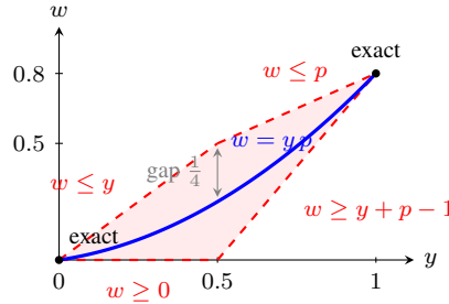
Figure 4: McCormick envelope of the bilinear term w = yp on the unit box, drawn along the slice p = 0.2 + 0.6y so that all four inequalities of (1) are distinct lines: the upper pair w \leq y , w \leq p forms the roof and the lower pair w \geq 0 , w \geq y + p - 1 the floor of the shaded feasible region, and the true product (blue) lies inside, touching the envelope only at the integer corners y \in \{0, 1\} . The largest over-credit is \frac{1}{4} , attained at y = p = \frac{1}{2} .
