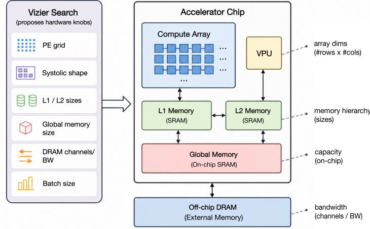
Figure 11: The accelerator datapath configuration. Processing elements (PEs) are arranged in a grid connected by a mesh network. Each PE contains a systolic array for matrix operations, a vector processing unit (VPU) for non-MAC operations, and private or shared L1/L2 memory. A Global Memory serves as the on-chip scratchpad shared across all PEs.
