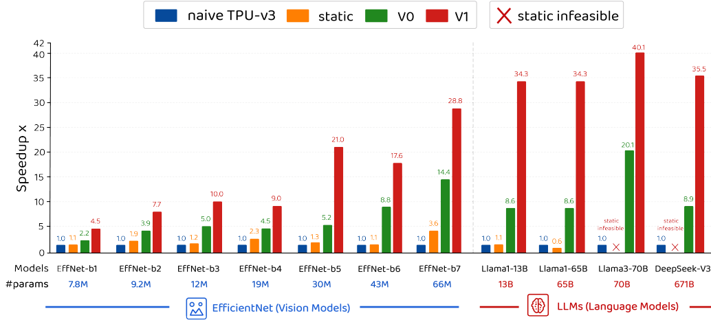
Figure 2: Speedup over modeled TPU-v3 baseline for each workload and formulation: CHEETAH-V1’s joint tiling–fusion optimization achieves up to \sim 40.1\times acceleration, while static fusion is infeasible on large-scale LLMs. Progressive gains are visible across formulations: V0’s dynamic placement improves over static by 2–20 \times , while V1’s joint tiling–fusion adds another 2–4 \times on top. See Section 6 for full analysis and wall-clock time breakdowns.
