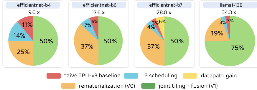
Figure 5: Speedup decomposition over naive TPU-v3 baseline. Each pie shows the relative contribution of four optimization sources to the total speedup. CHEETAH-V1 joint tiling + fusion dominates on all workloads, especially on larger models where memory management is the primary bottleneck.
