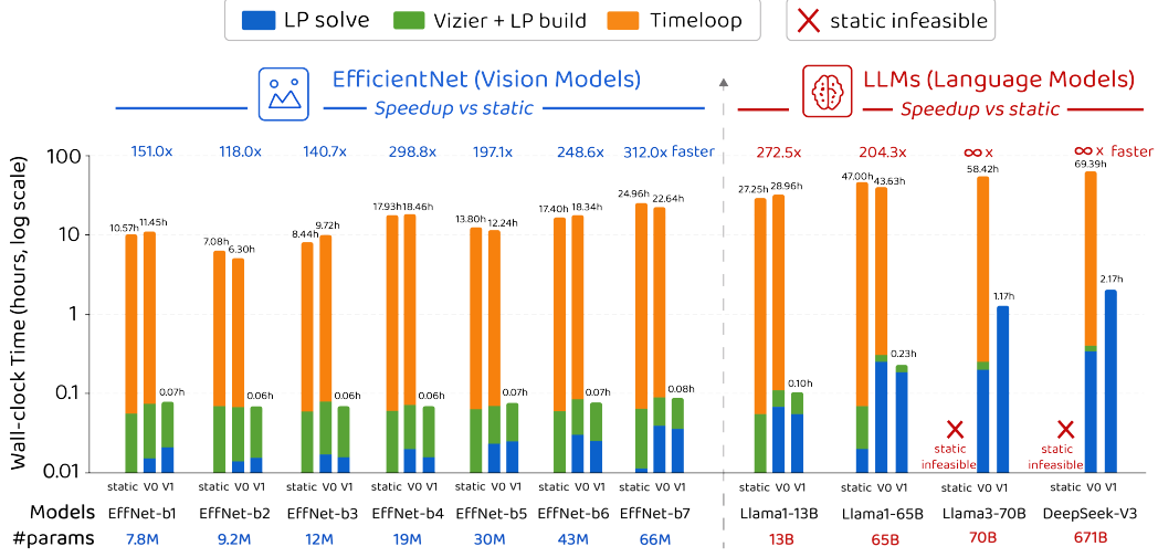
Figure 6: Wall-clock time decomposition and performance acceleration across formulations: CHEETAH-V1’s internalized tiling eliminates the Timeloop bottleneck, achieving up to 100–300× faster search than the classical static method. Upper bars show wall-clock hours (log scale); annotations show speedup vs. static.
