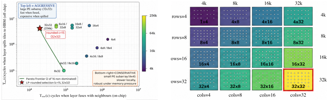
Figure 7: Example per-layer tiling cache for EfficientNet-B7 layer L4. Left: Timeloop-evaluated candidates plotted by fused/on-chip cost T_{\min}(c) and spilled/off-chip cost T_{\max}(c) ; the frontier shows non-dominated choices and the star is the LP-rounded selection. Right: the 16 tiling choices; labels such as 4 \times 4 , 8 \times 8 , and 32 \times 32 denote active tile rows/columns inside the fixed accelerator, white dots indicate active PE/MAC sites. These are schedule choices, not different chips.
