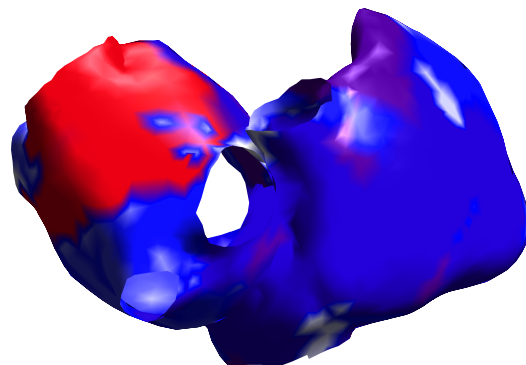
Interpolation
