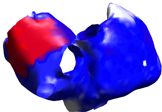
Ground Truth
